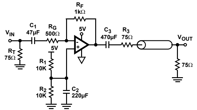
FIGURE 36. SINGLE SUPPLY INVERTING VIDEO LINE DRIVER
