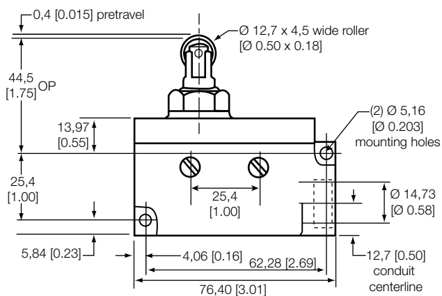
Figure 15. E7S Series, inline roller plunger, side mount
