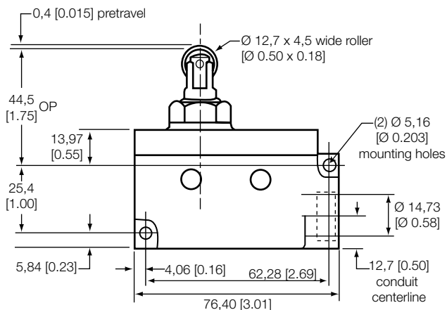
Figure 7. E7 Series, inline roller plunger, diagonal mount
