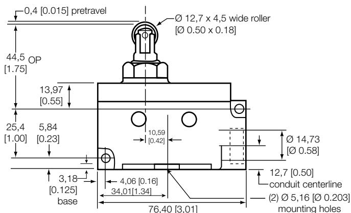
Figure 29. V7 Series, inline roller plunger, flange mount
