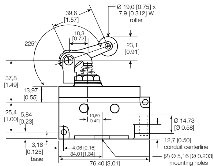
Figure 31. V7 Series, roller lever, flange mount
