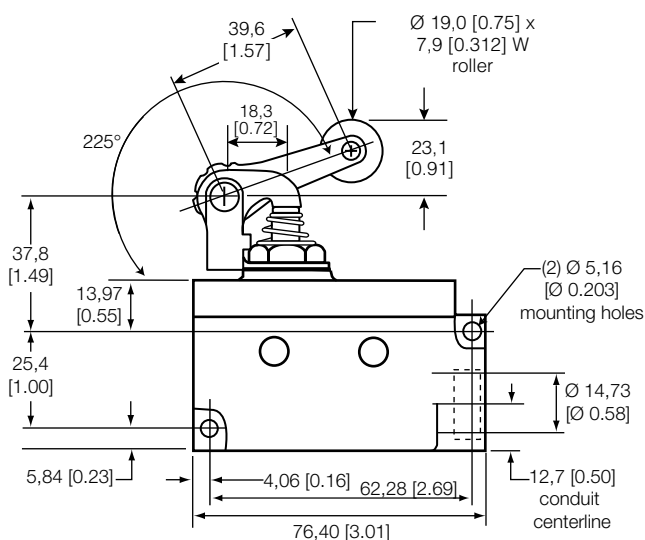
Figure 9. E7 Series, roller lever, diagonal mount
