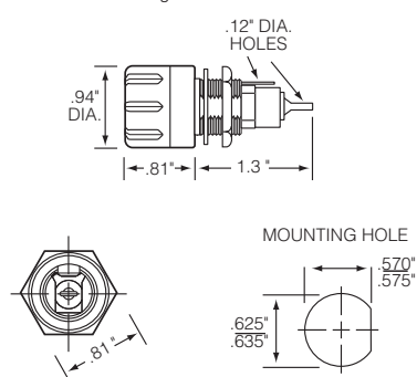
Watertight Product Dimensions
