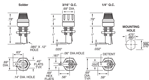
General Application / Right Angle Terminal Product Dimensions
