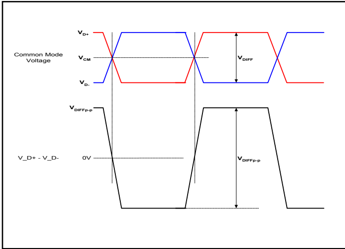
Definition of Differential Voltage and Differential Voltage Peak-to-Peak
