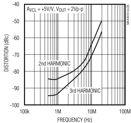
MAX4415/MAX4417/MAX4419 DISTORTION vs. FREQUENCY
