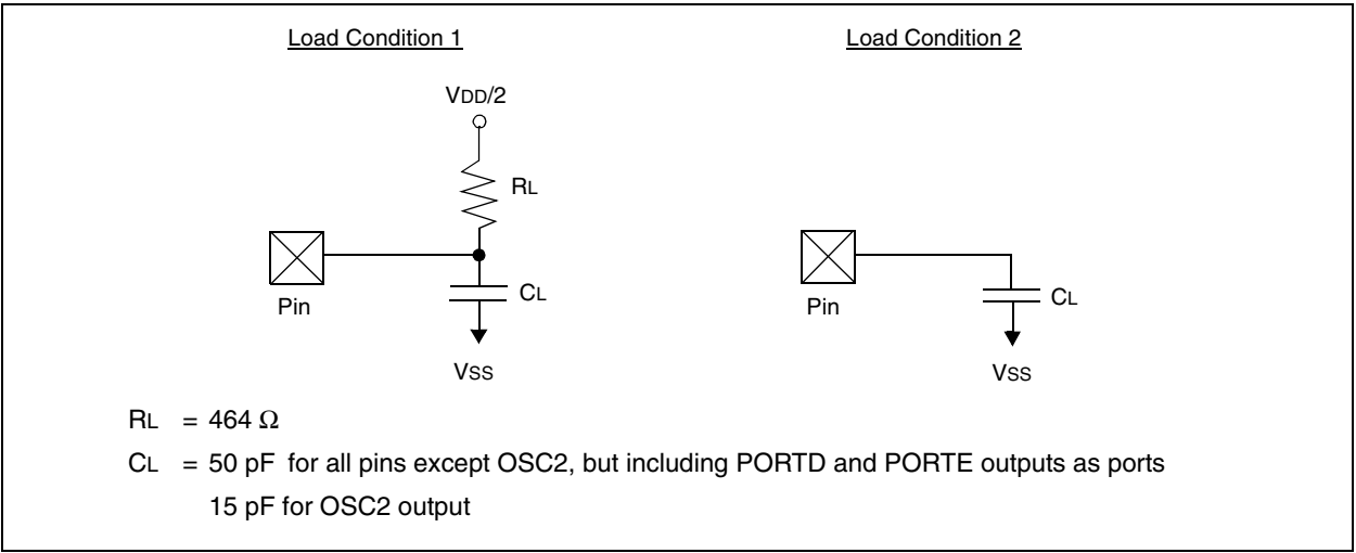
FIGURE 14-3: LOAD CONDITIONS
