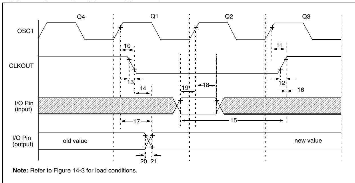
FIGURE 14-5: CLKOUT AND I/O TIMING
