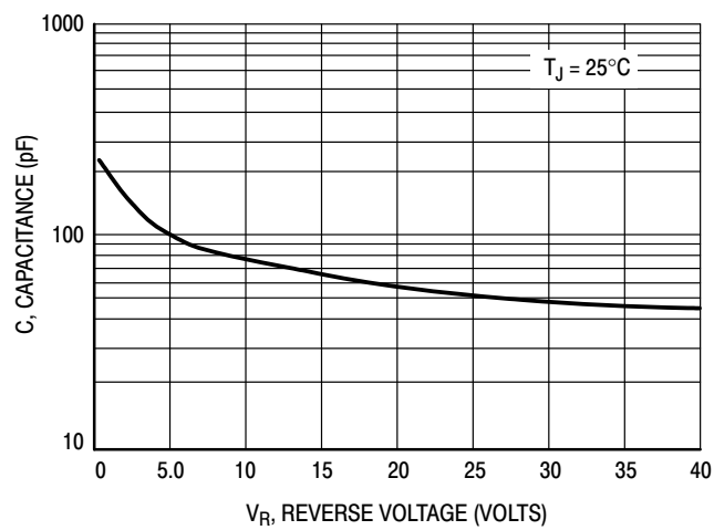
Figure 5. Capacitance
