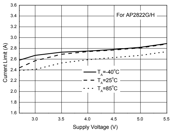
Figure 14. Current Limit vs. Supply Voltage
