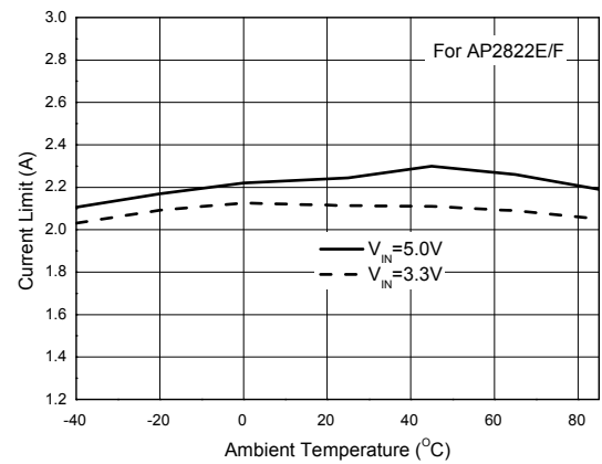
Figure 13. Current Limit vs. Ambient Temperature
