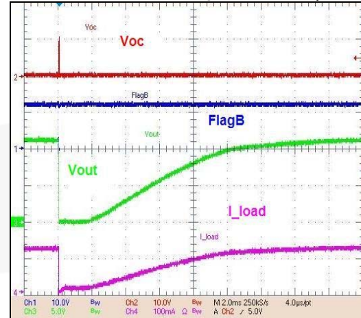
Figure 35. OUT Shorted to GND, Short Condition Removed (SOA Protection Followed by a Normal Operation, FPF2700 / FPF2701)
