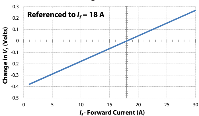
Forward Voltage vs Forward Current
