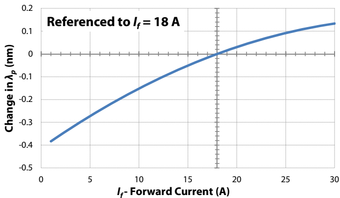
Peak Wavelength vs Forward Current
