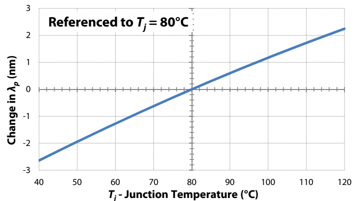
Peak Wavelength vs Junction Temperature
