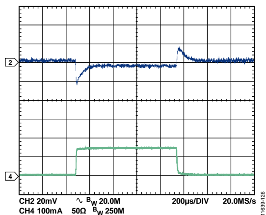
Figure 32. VREG2 Load Transient, V_{REG2} = 3.3\text{ V}
