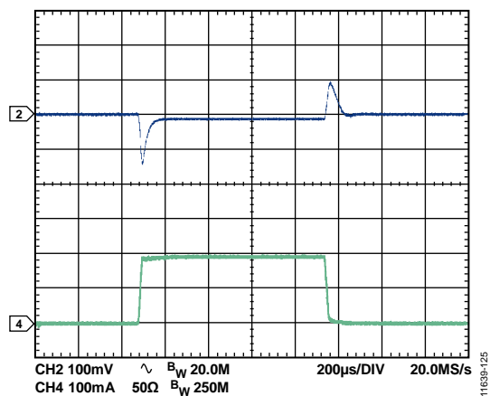
Figure 31. VREG1 Load Transient, V_{REG1} = 5\text{ V}
