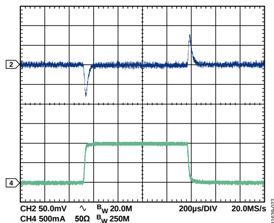
Figure 27. Channel 5 Load Transient, V_{OUT} = 3.3 V, PPWM Mode
