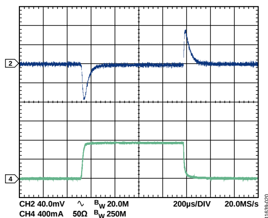
Figure 23. Channel 3 Load Transient, V_{OUT} = 1.8 V, PPWM Mode
