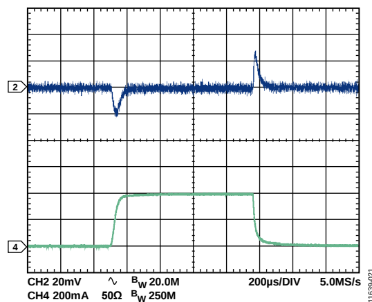
Figure 25. Channel 4 Load Transient, V_{OUT} = 3.3 V, PPWM Mode
