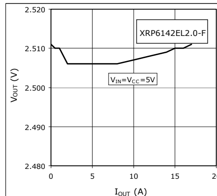
Fig. 7: Load regulation
