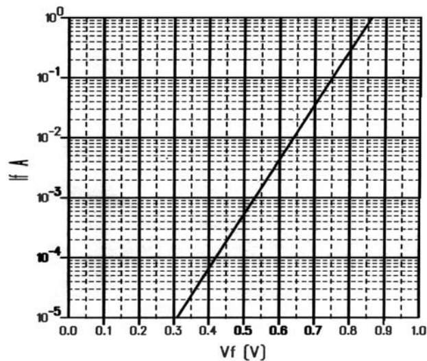
UM4000/UM4900 TYPICAL
