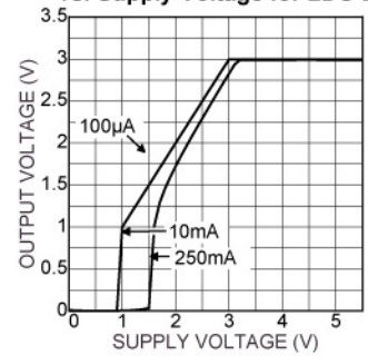
Output Voltage vs. Supply Voltage for LDO 2
