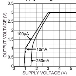
Output Voltage vs. Supply Voltage for LDO 1
