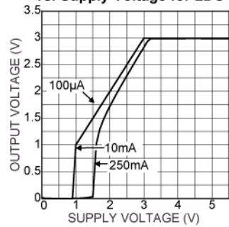
Output Voltage vs. Supply Voltage for LDO 3
