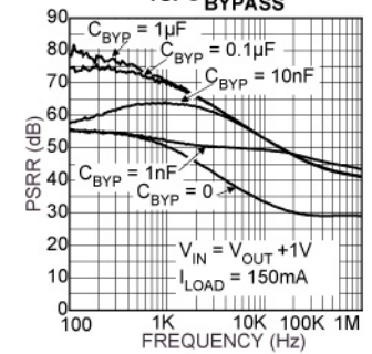
Power Supply Rejection Ratio vs. C_{BYPASS}
