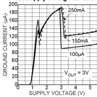
Ground Current vs. Supply Voltage for LDO 3
