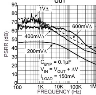
Power Supply Rejection Ratio vs. 3V_{OUT}
