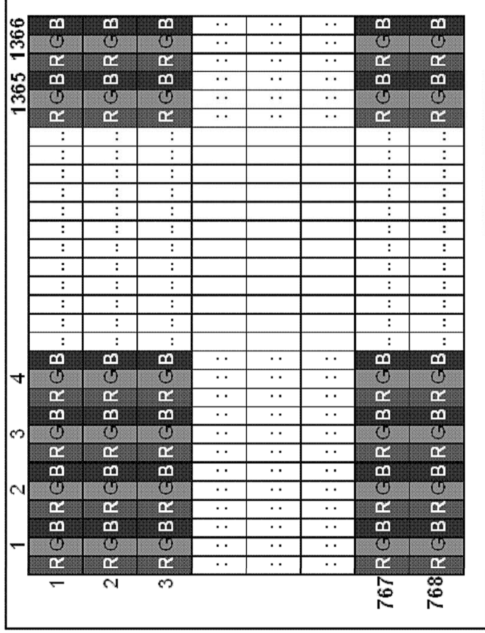
Figure 2 Pixel Format
