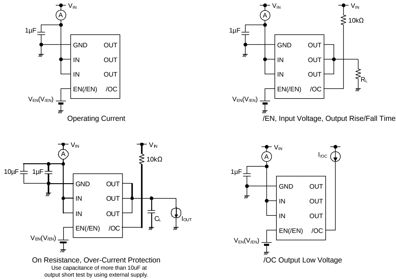
Figure 4. Measurement Circuit
