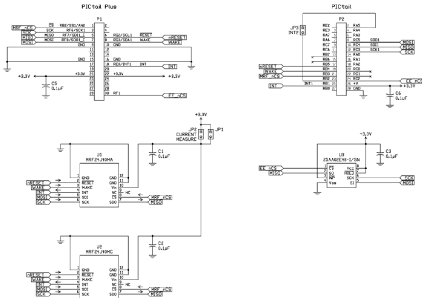
FIGURE A-1: MRF24J40MC PICTail™/PICTail PLUS DAUGHTER BOARD SCHEMATIC
