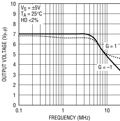
Undistorted Output Swing vs Frequency ( \pm 5V )
