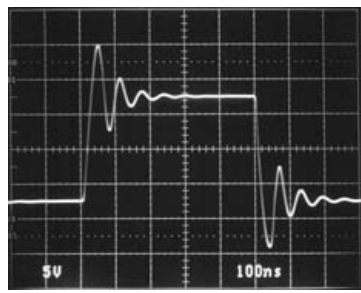
Large-Signal Transient (Noninverting, G = 1, C_L = 100pF )
