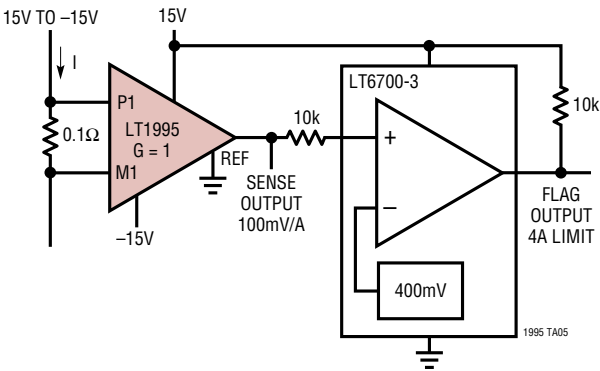
Current Sense with Alarm
