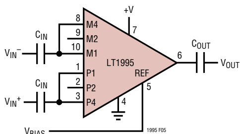
Figure 5. AC-Coupled Difference Amplifier General Configuration (G = 5 Example)
