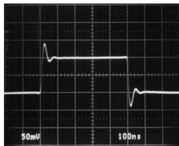
Small-Signal Transient (G = -1)
