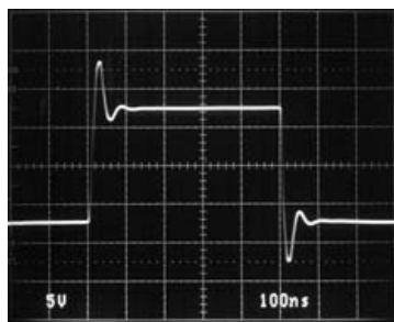
Large-Signal Transient (G = -1)
