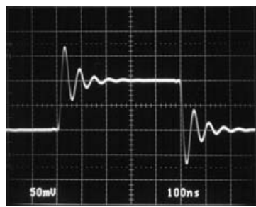
Small-Signal Transient (Noninverting, G = 1, C_L = 100pF )
