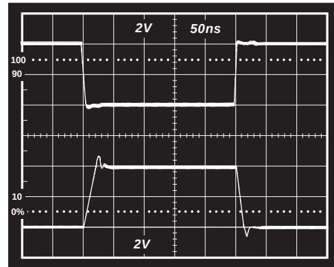
TPC 23. Inverter Large Signal Pulse Response; V_S = \pm 5V , C_F = 1pF , R_L = 1k\Omega
