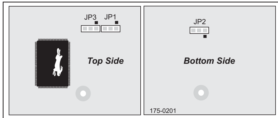
Figure A-6. Location of RCM2000 Configurable Positions
