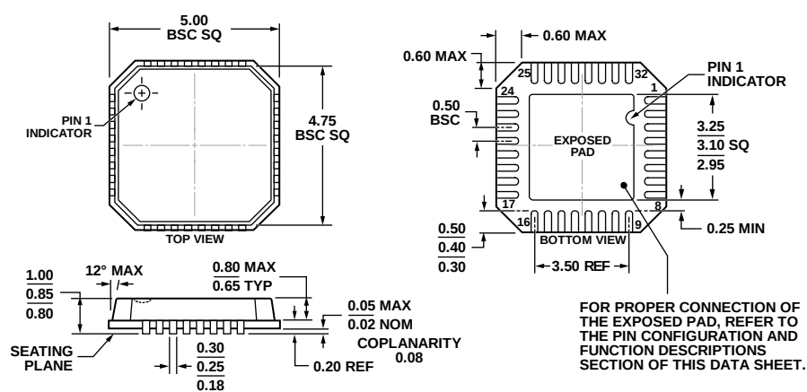
Figure 85. 32-Lead Lead Frame Chip Scale Package [LFCSP_VQ] 5 mm x 5 mm Body, Very Thin Quad (CP-32-2) Dimensions shown in millimeters
