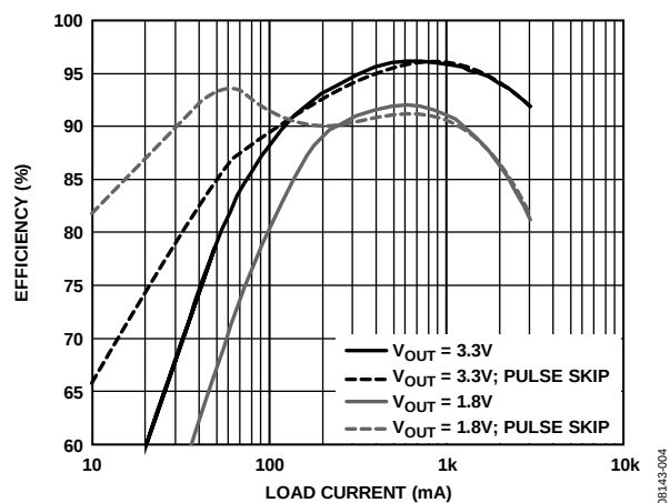
Figure 4. Channel 1 Efficiency vs. Load, V_{IN} = 5\text{ V} and f_{SW} = 300\text{ kHz} ; V_{OUT} = 3.3\text{ V} , Inductor Cooper Bussmann DR1050-8R2-R, 8.2\text{ }\mu\text{H} , 15\text{ m}\Omega ; V_{OUT} = 1.8\text{ V} , Inductor TOKO FDV0620-4R7M, 4.7\text{ }\mu\text{H} , 53\text{ m}\Omega
