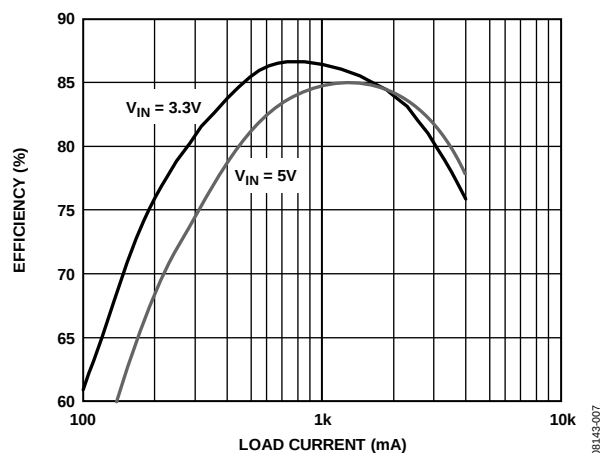
Figure 7. Efficiency Combined Dual-Phase Output, V_{OUT} = 0.8\text{ V} and f_{SW} = 1.2\text{ MHz} ; Inductor TOKO FDV0620-1R0M, 1.0\text{ }\mu\text{H} , 14\text{ m}\Omega
