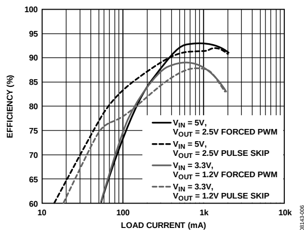
Figure 6. Efficiency vs. Load at f_{SW} = 1.2\text{ MHz} ; Inductor TOKO FDV0620-1R0M, 1.0\text{ }\mu\text{H} , 14\text{ m}\Omega
