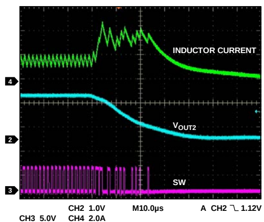
Figure 55. Current Limit Entry (Zoomed In), Channel 2 V_{OUT} = 1.8\text{ V} , 2 A Configuration, f_{SW} = 600\text{ kHz}
