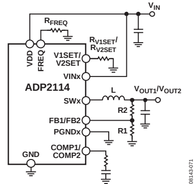
Figure 71. Configuration for Adjustable Outputs
