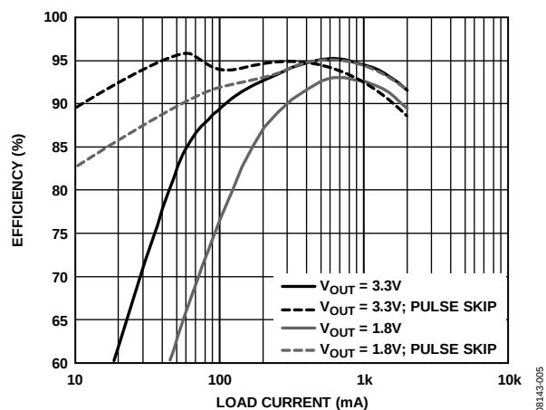
Figure 5. Channel 2 Efficiency vs. Load, V_{IN} = 5\text{ V} and f_{SW} = 600\text{ kHz} ; V_{OUT} = 3.3\text{ V} , Inductor TOKO FDV0620-4R7M, 4.7\text{ }\mu\text{H} , 53\text{ m}\Omega ; V_{OUT} = 1.8\text{ V} , Inductor TOKO FDV0620-2R2M, 2.2\text{ }\mu\text{H} , 30\text{ m}\Omega
