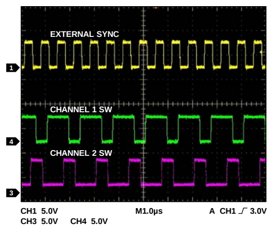
Figure 58. External Synchronization, f_{\text{SYNC}} = 1.5 \text{ MHz} , f_{\text{SW}} = 750 \text{ kHz}
