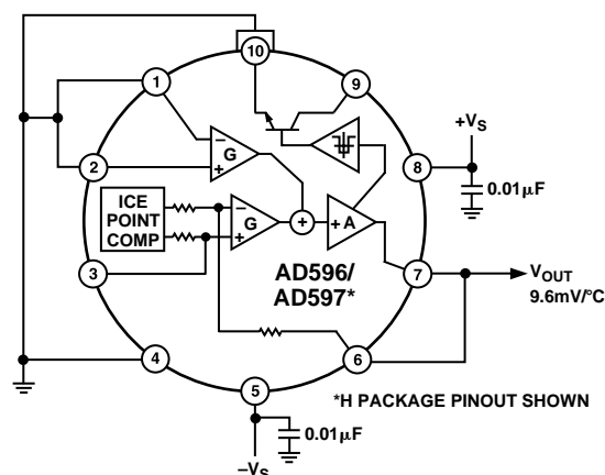
Figure 3. Stand-Alone Temperature Transducer Temperature Proportional Output Connection
