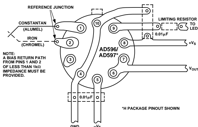
Figure 4. PCB Connections
