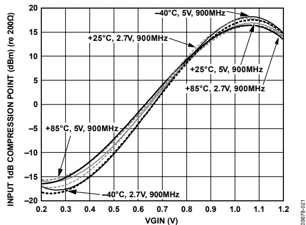
Figure 21. Input 1 dB Compression Point (IP1dB) vs. V_{GIN} , F_{IF} = 900\text{ MHz} , F_{BB} = 1\text{ MHz} , V_{POS} = 2.7\text{ V} , 5\text{ V} , Temperature = -40^{\circ}\text{C} , +25^{\circ}\text{C} , +85^{\circ}\text{C}
