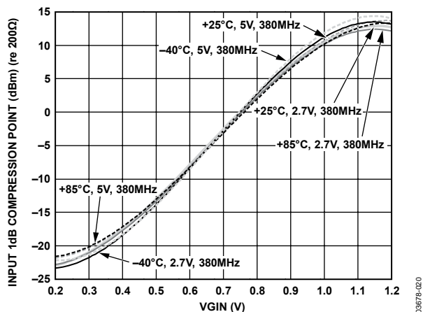
Figure 20. Input 1 dB Compression Point (IP1dB) vs. V_{GIN} , F_{IF} = 380\text{ MHz} , F_{BB} = 1\text{ MHz} , V_{POS} = 2.7\text{ V} , 5\text{ V} , Temperature = -40^{\circ}\text{C} , +25^{\circ}\text{C} , +85^{\circ}\text{C}
