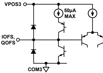
Figure 8. Circuit F
