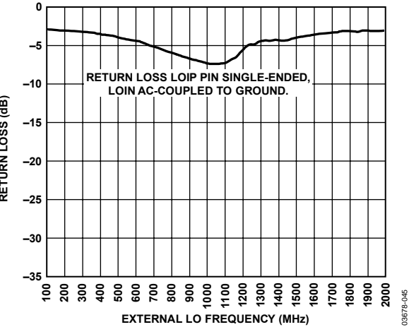
Figure 45. Return Loss of LOIP Input vs. External LO Frequency
