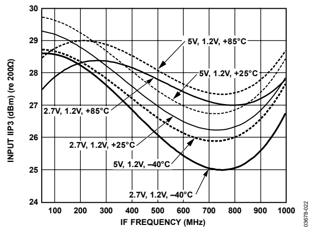
Figure 22. IIP3 vs. F_{IF} , V_{GIN} = 1.2\text{ V} , F_{BB} = 1\text{ MHz} , V_{POS} = 2.7\text{ V} , 5\text{ V} , Temperature = -40^{\circ}\text{C} , +25^{\circ}\text{C} , +85^{\circ}\text{C} , Tone Spacing = 20\text{ kHz}
