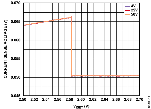
Figure 14. Current Sense Voltage vs. ISET Voltage ( V_{ISET} ), Different Input Voltages
