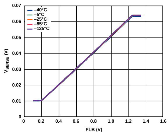
Figure 27. Sense Voltage ( V_{SENSE} ) vs. FLB, Different Temperatures
