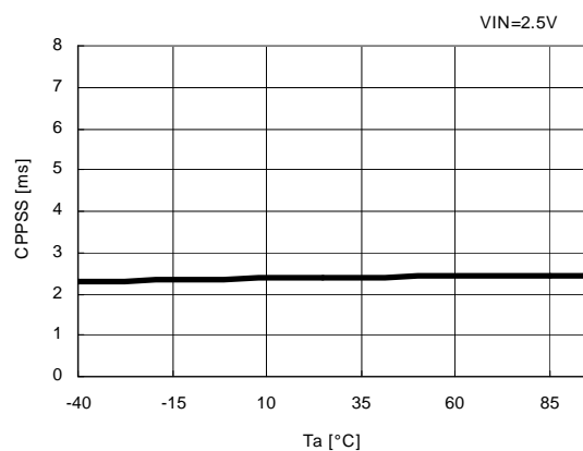
22) CPP Soft-Start VS. Temperature R1290K102A
