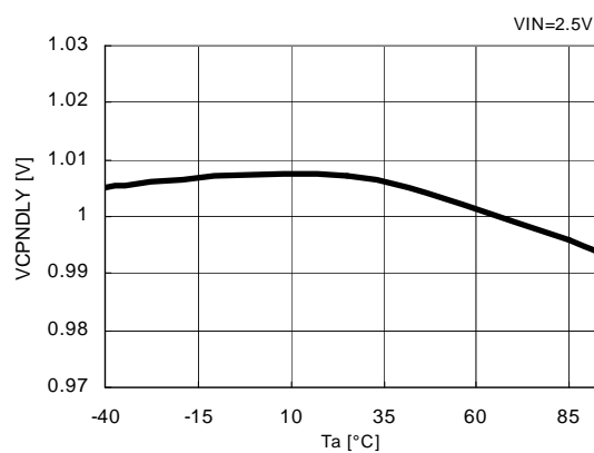
27) CPNDLY Detector Threshold VS. Temperature R1290K102A
