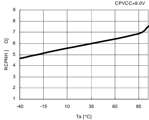
32) CPN" H "ON Resistance VS. Temperature R1290K102A
