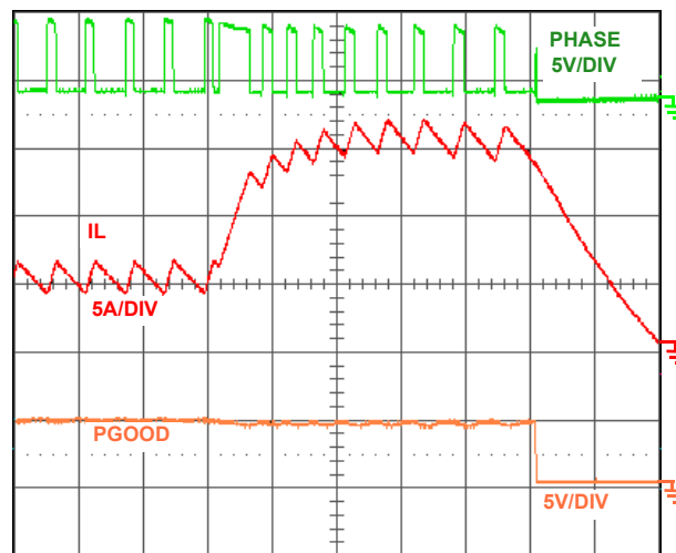
FIGURE 22. OVERCURRENT SHUTDOWN
