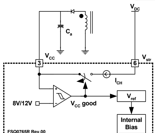
Figure 31. Startup Circuit
