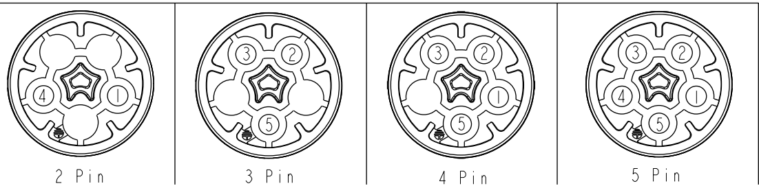
Pin Assignments Front View
