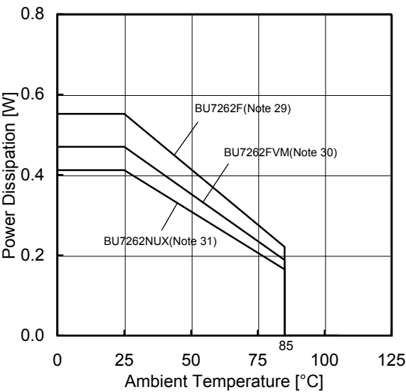
(e)BU7262F/FVM/NUX
