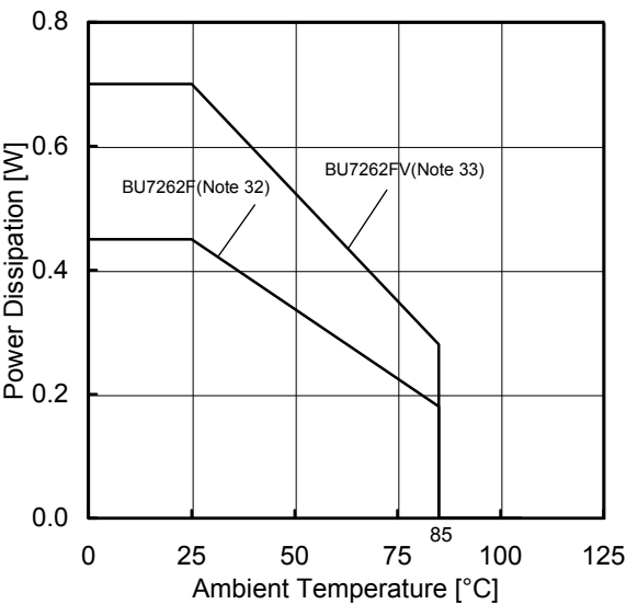
(g)BU7264F/FV
