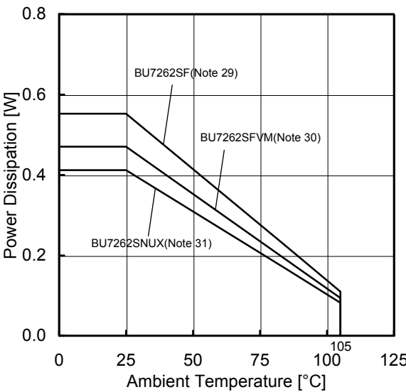
(f)BU7262SF/SFVM/SNUX
