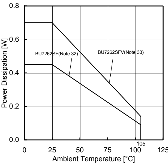
(h)BU7264SF/SFV
