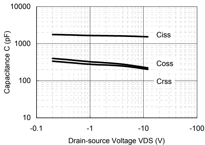
Capacitance - VDS
