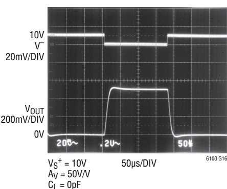
Step Response at V_{SENSE} = 0\text{V} to 10\text{mV}
