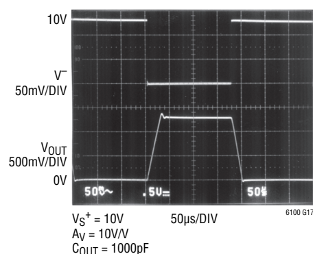
Step Response at V_{SENSE} = 0\text{V} to 130\text{mV}
