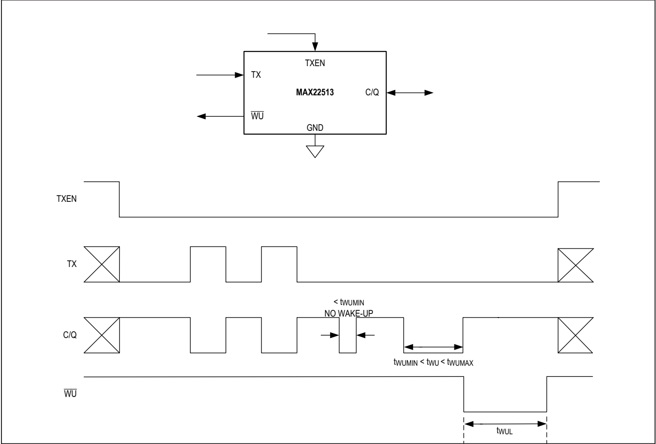
Figure 5. Wake-Up Timing
