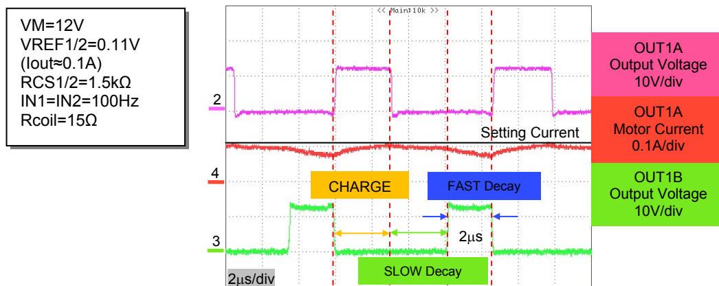
Figure 32. One full PWM cycle of the constant-current control
