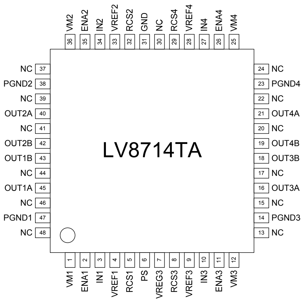
Figure 5. Pin Assignment
