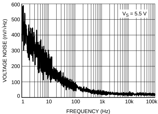
Figure 11. Input Voltage Noise vs. Frequency
