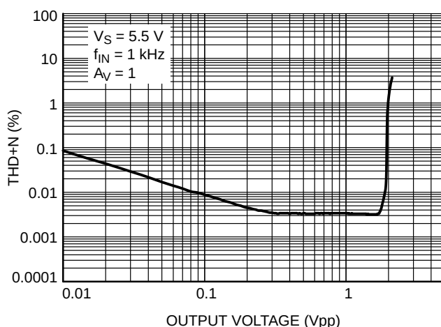
Figure 9. THD + N vs. Output Voltage
