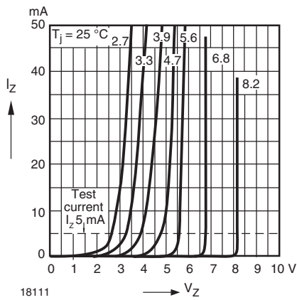
Fig. 14 - Breakdown Characteristics
