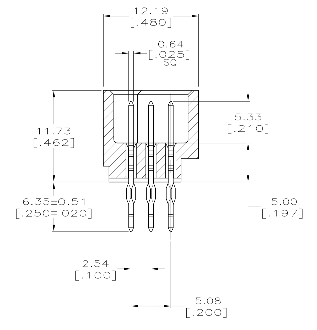
SECTION T-T
