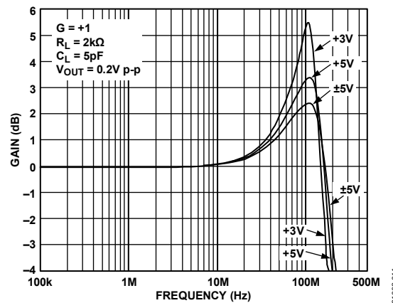
Figure 11. AD8054 Gain vs. Frequency vs. Supply
