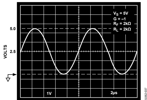
Figure 37. Output Swing; G = -1 , R_L = 2 \text{ k}\Omega
