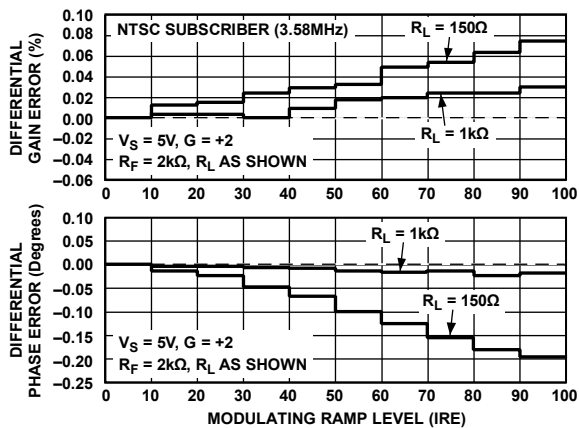
Figure 21. AD8051/AD8052 Differential Gain and Phase Errors
