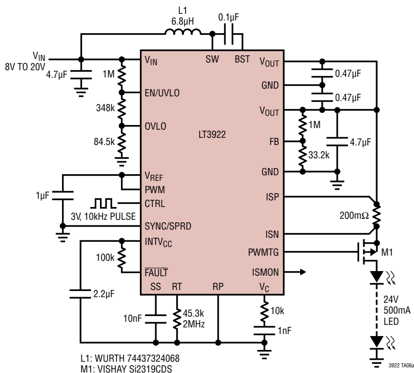
500mA Boost LED Driver Using Pulse Duty Cycle CTRL Input
