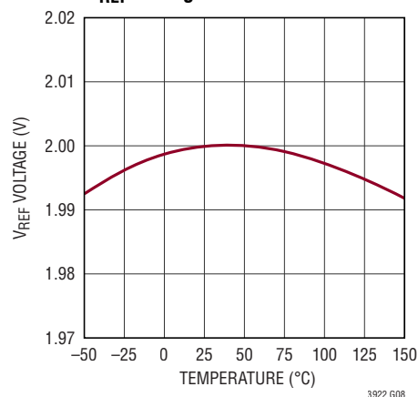
V_{REF} Voltage
