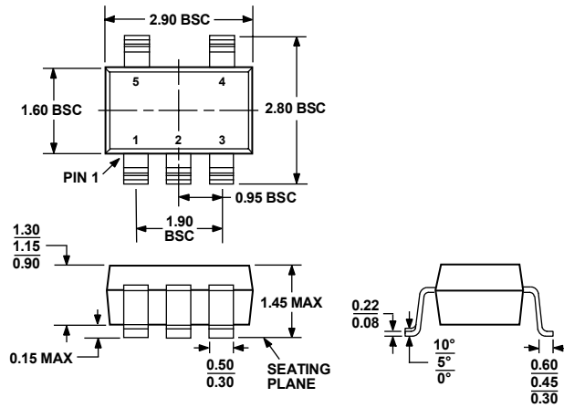
Figure 33. 5-Lead Small Outline Transistor Package [SOT-23] (RJ-5) Dimensions shown in millimeters
