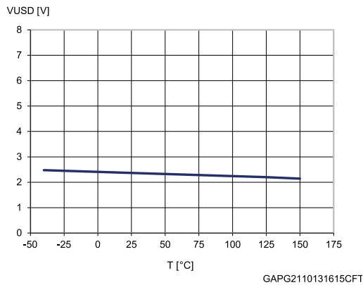
Figure 19: Undervoltage shutdown
