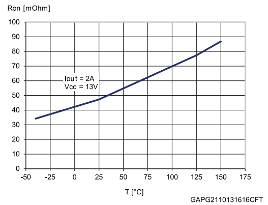
Figure 20: On-state resistance vs. Tcase
