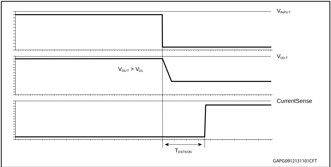
Figure 8: TDSTKON
