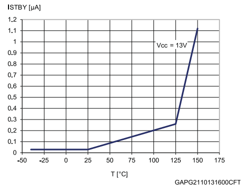
Figure 12: Standby current
