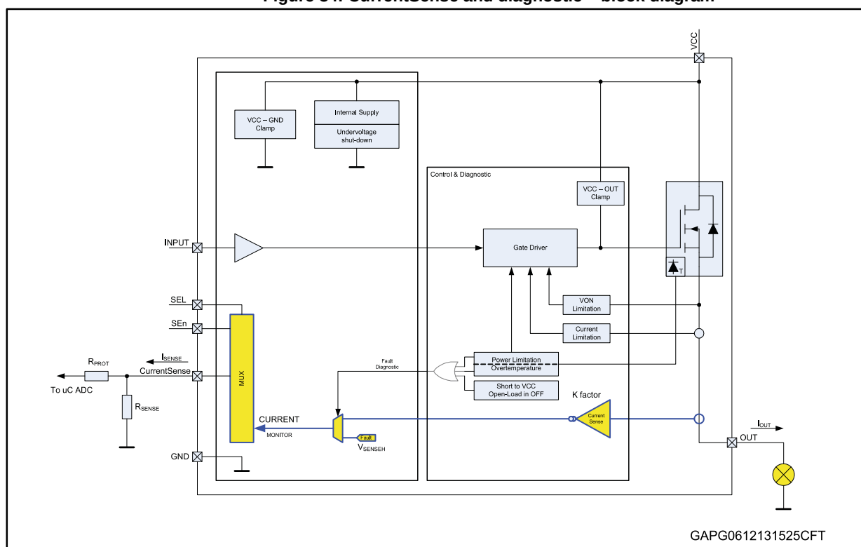
Figure 34: CurrentSense and diagnostic – block diagram
