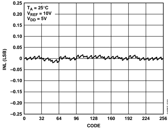
Figure 6. INL vs. Code (8-Bit DAC)
