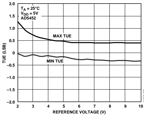
Figure 20. TUE vs. Reference Voltage
