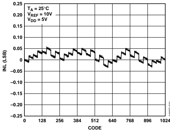
Figure 7. INL vs. Code (10-Bit DAC)
