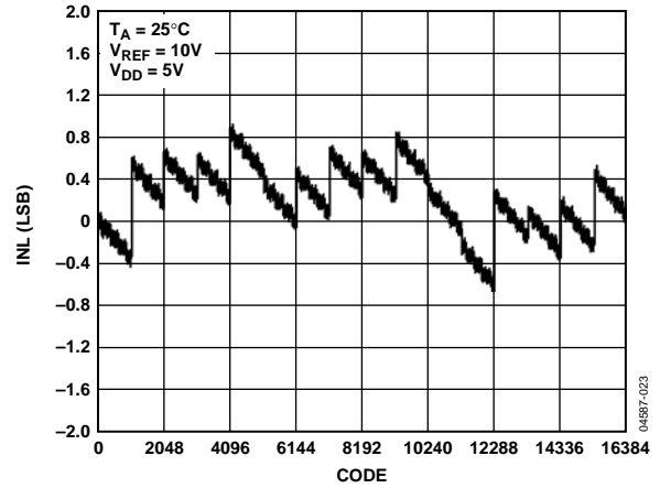
Figure 9. INL vs. Code (14-Bit DAC)
